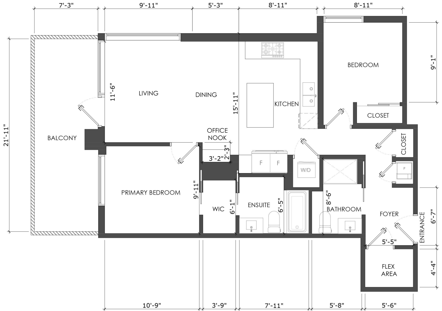
MAIN FLOOR PLAN Ceiling Height: 9'-0"
